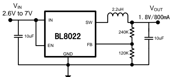
1.8V/800mA Step-Down Converter
